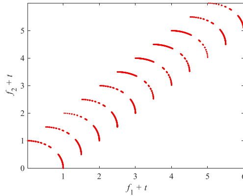
Fig. 6 Illustration of the true PF of DCF6.
